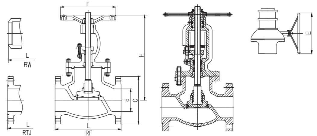
Dimensions and Weights 尺寸及重量 (Class150 ~ Class900)
